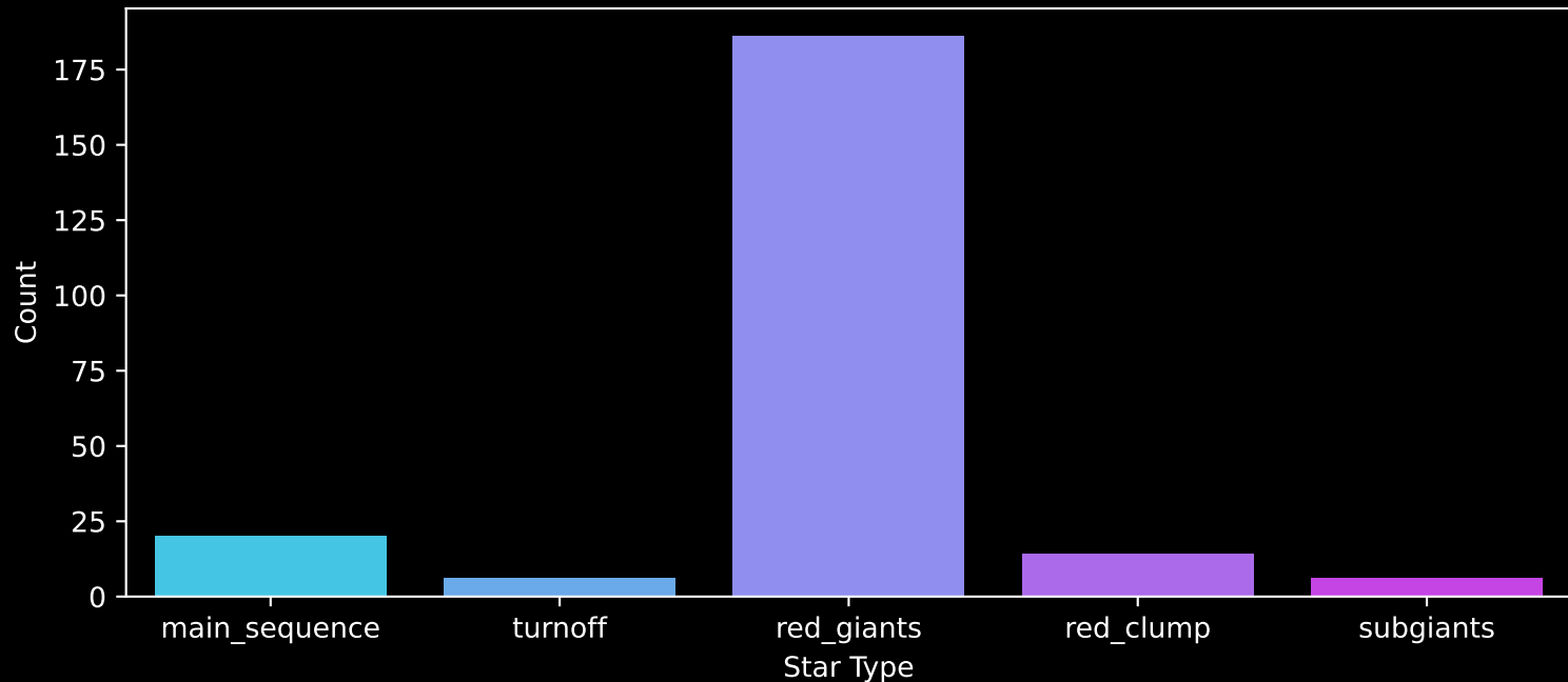
APOGEE DR17 Field: [Tombaugh2] Count plot of Star Type
