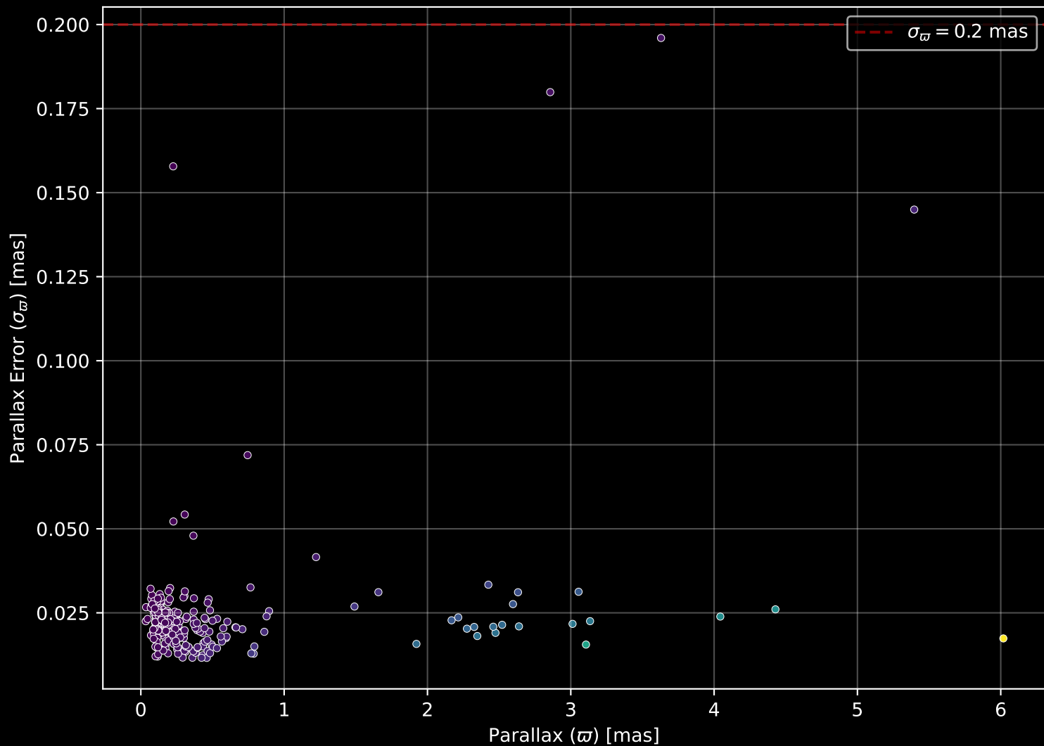
APOGEE DR17 Field: [Tombaugh2] Parallax Quality (n= 232)
