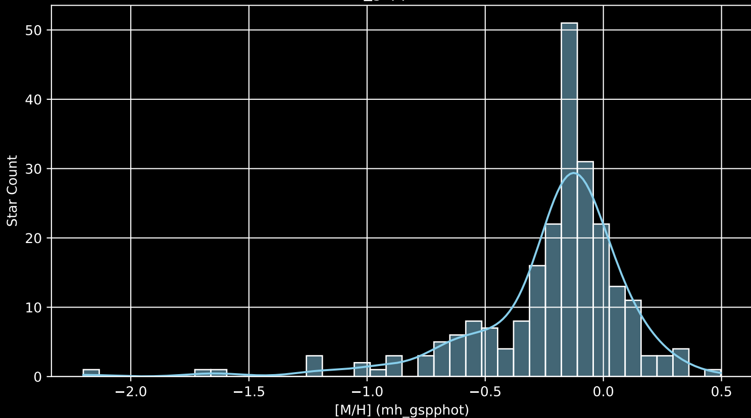
APOGEE DR17 Field: [Tombaugh2 [M/H] (mh_gspphot) (n= 230)
