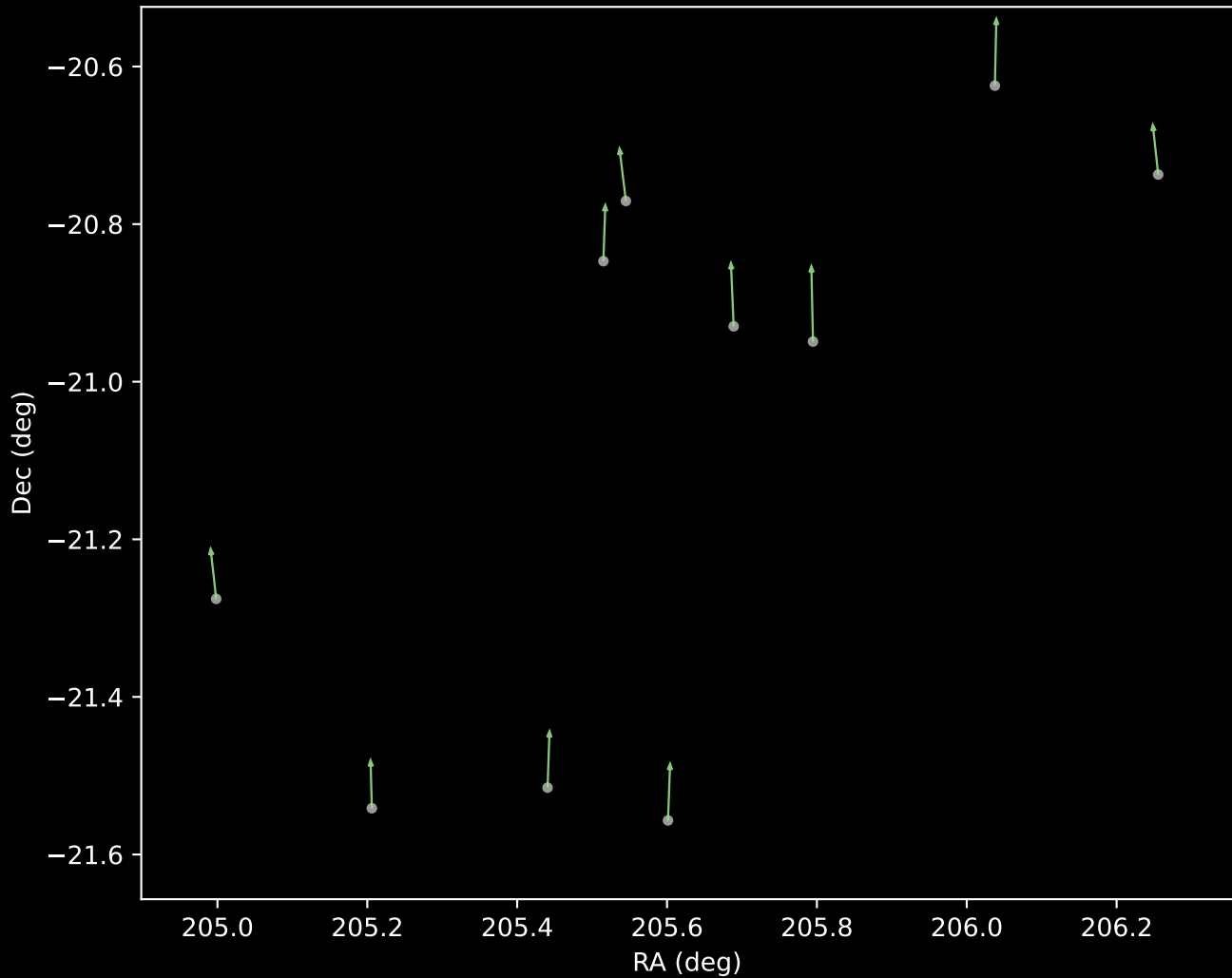
APOGEE DR17 Cluster 5 Proper Motion Vectors (n=10)
