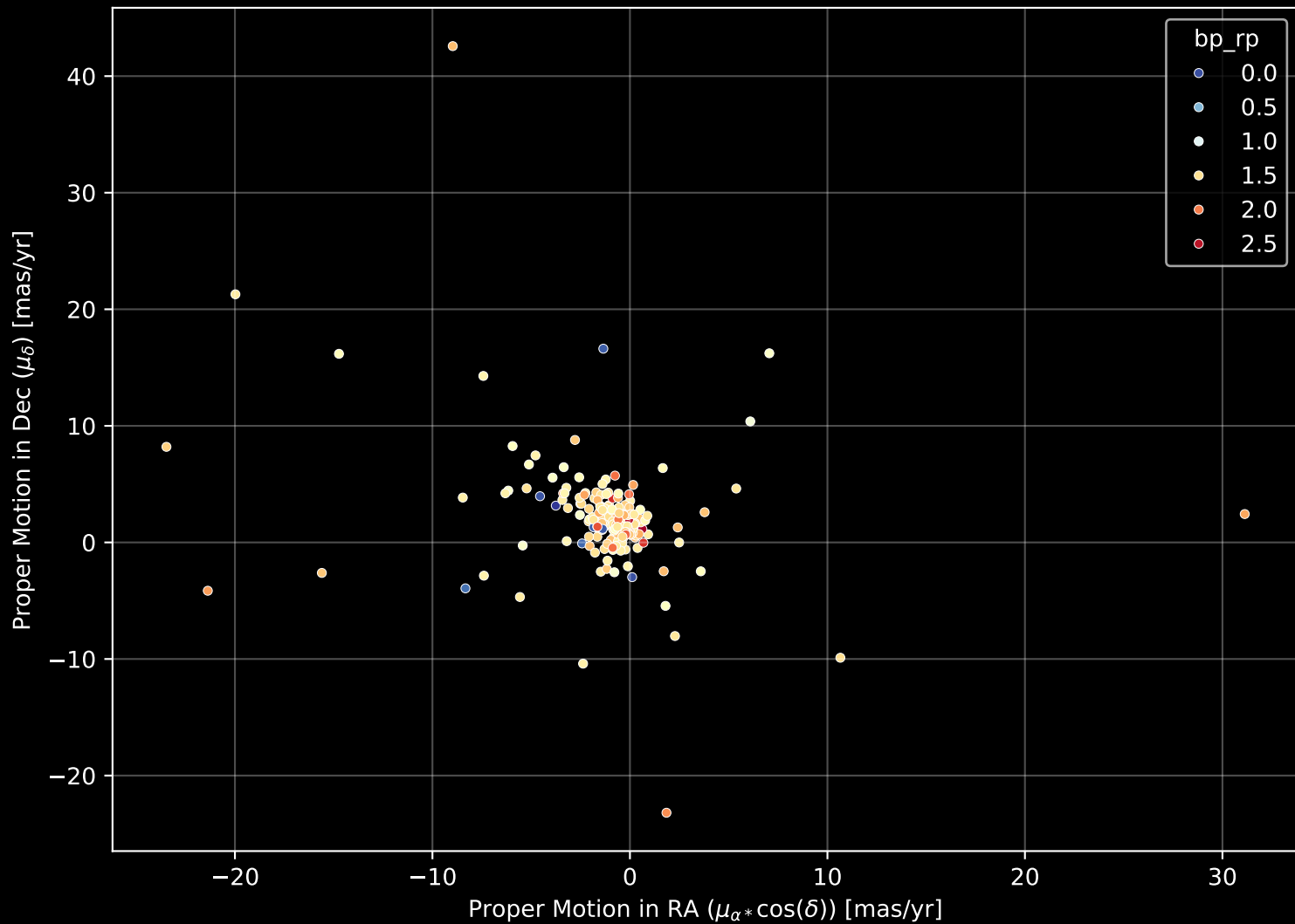
APOGEE DR17 Field: [Tombaugh2] Proper Motion Diagram (n= 232)
