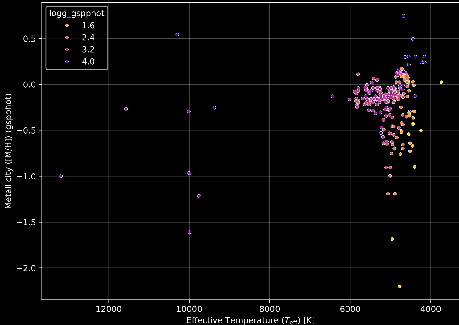
APOGEE DR17 Field: [Tombaugh2] Stellar Population Parameters (n= 232)
