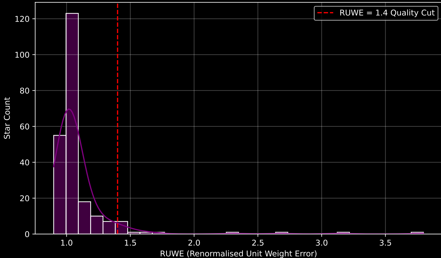
GAPOGEE DR17 Field [Tombaugh2] RUWE Distribution (n= 227)
