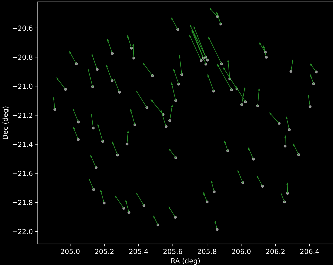
APOGEE DR17 Cluster 4 Proper Motion Vectors (n=69)
