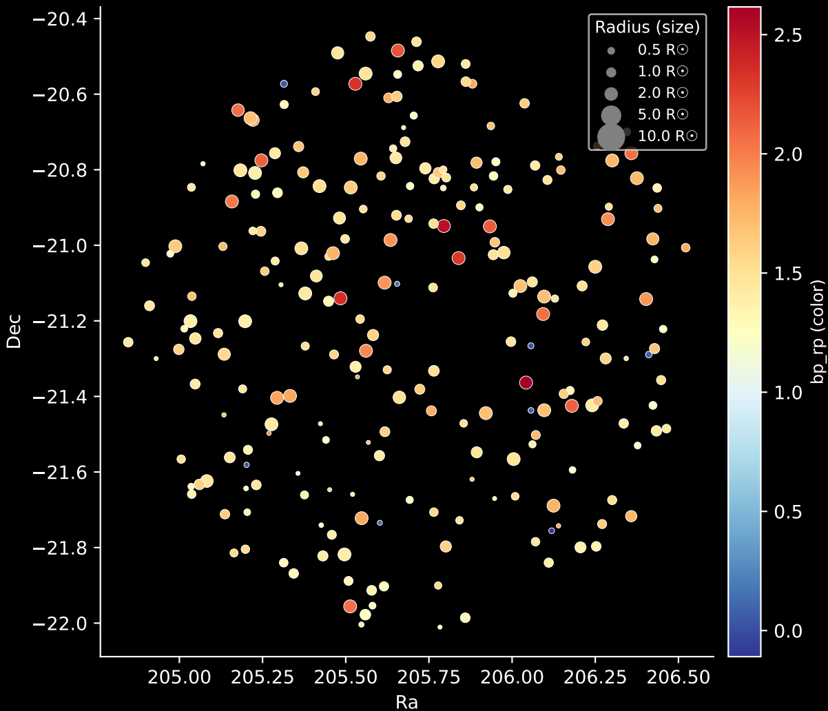
APOGEE DR17 Field: [Tombaugh2] Stars: 232
