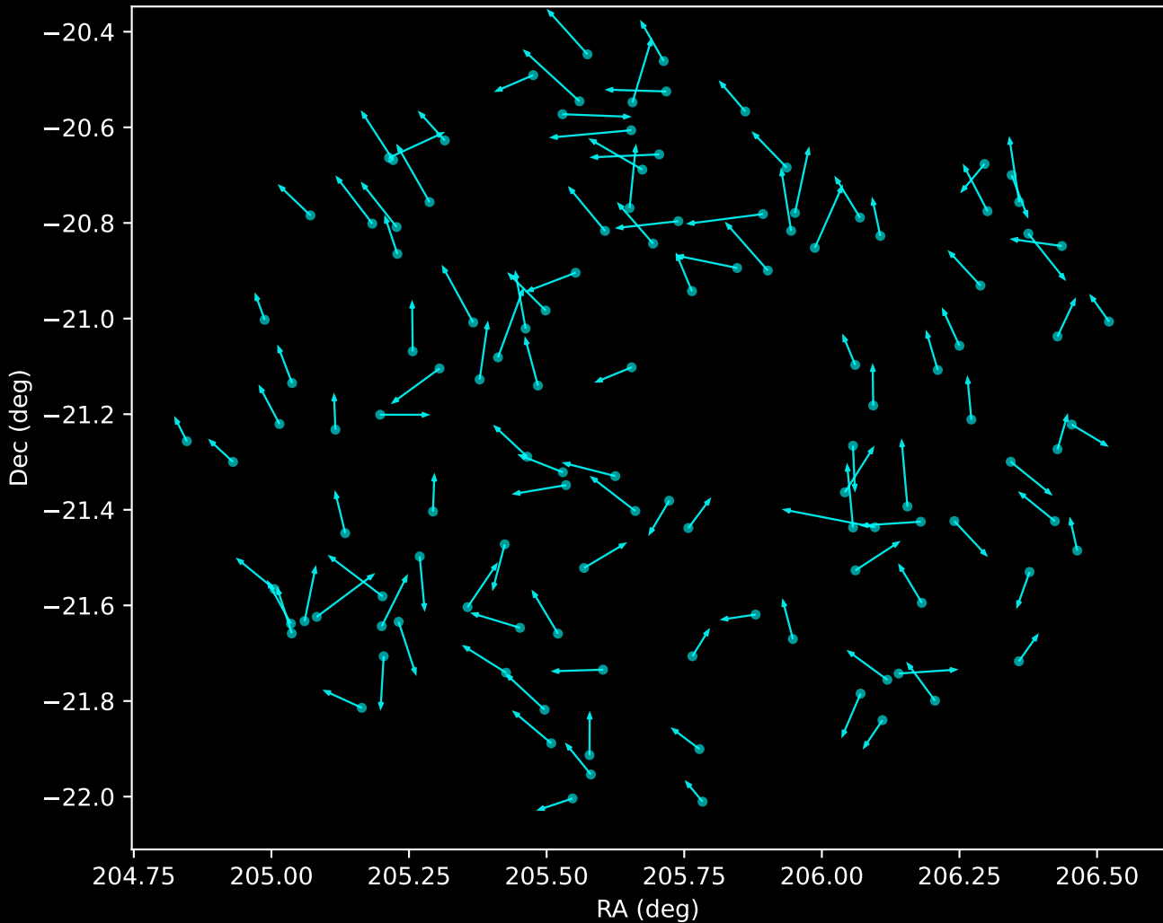
APOGEE DR17 Noise Stream Proper Motion Vectors (n=122)
